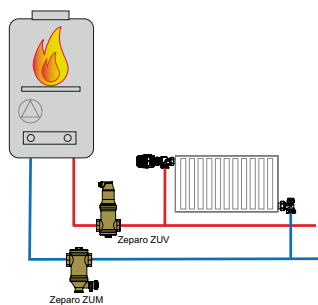
Cazan mural
