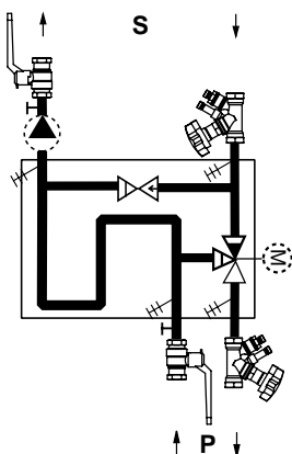
Prefabricated control loop 16
