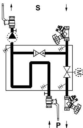
Prefabricated control loop 26
