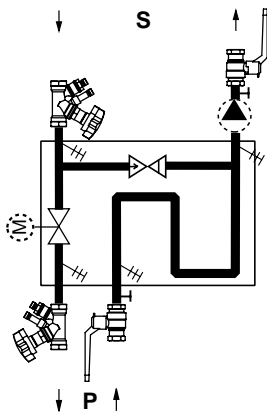
Prefabricated control loop 25
