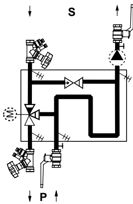
Prefabricated control loop 15
