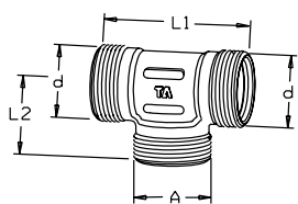
TA 352 Tee Male Non-plated (yellow)
